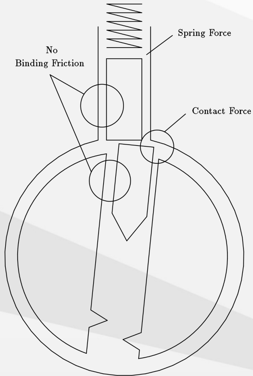
Figure 5.3: Pins at the sheer line
