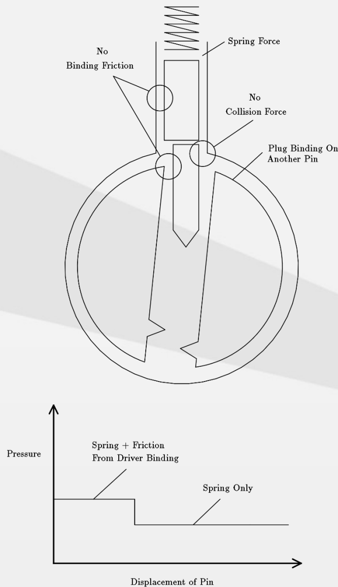
Figure 9.3: Driver pin wider than key pin
