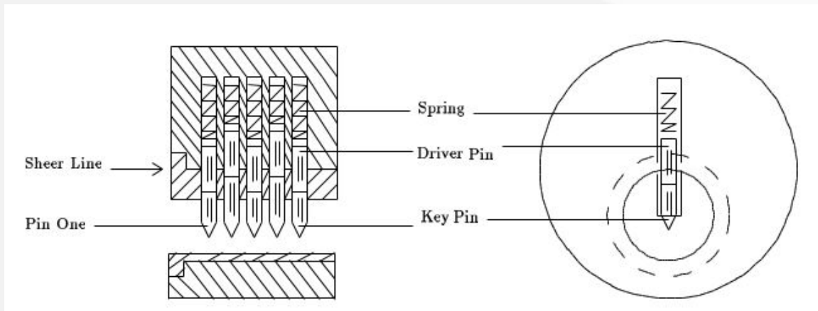
Figure 2.1: Workings of pin tumbler locks
