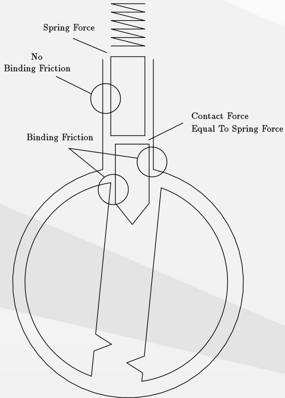
Figure 5.4: Key pin enters hull
