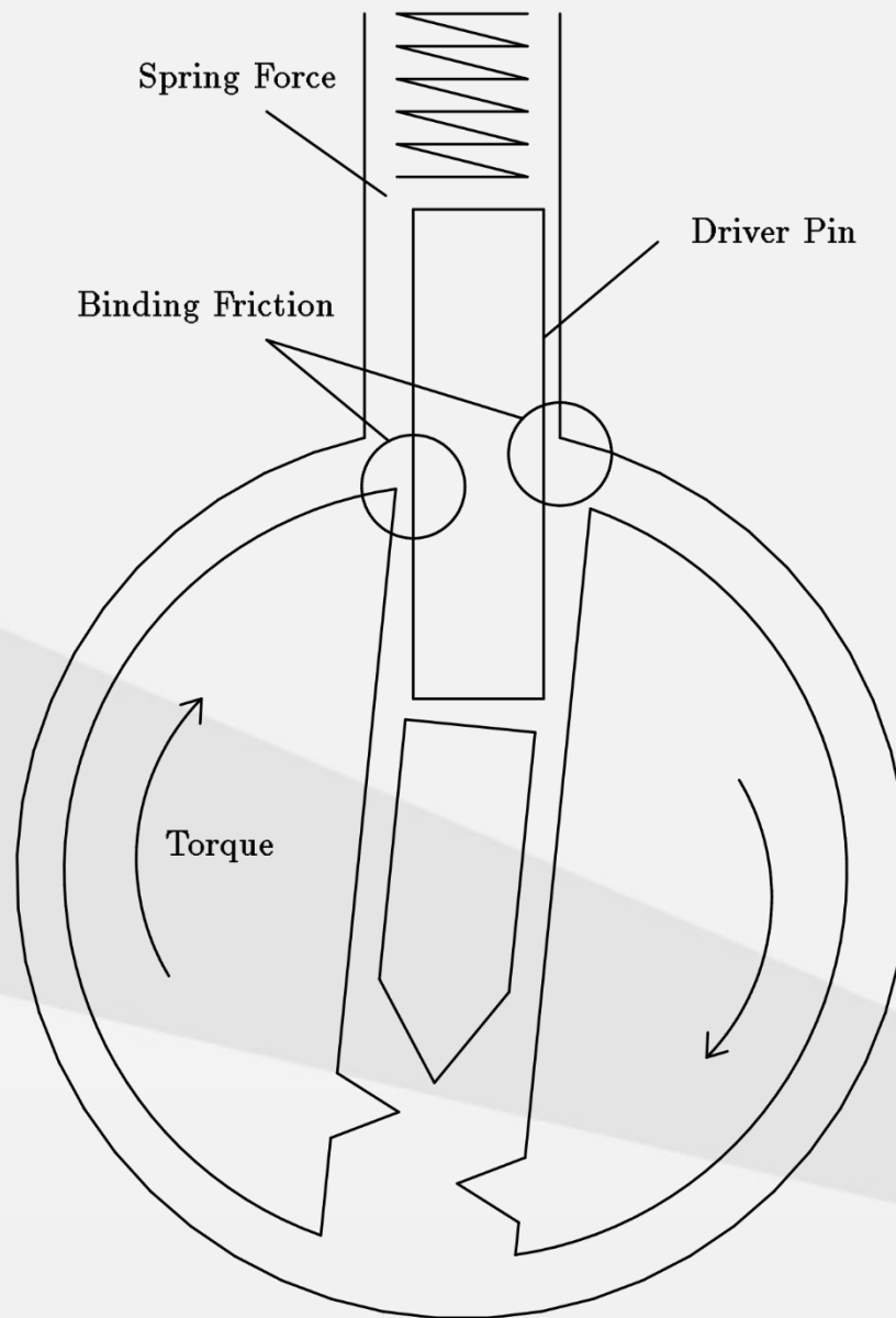
Figure 5.2: Binding in the pin-column model
