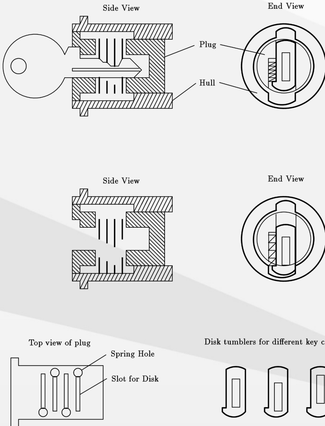
Figure 9.10: Workings of a disk tumbler lock
