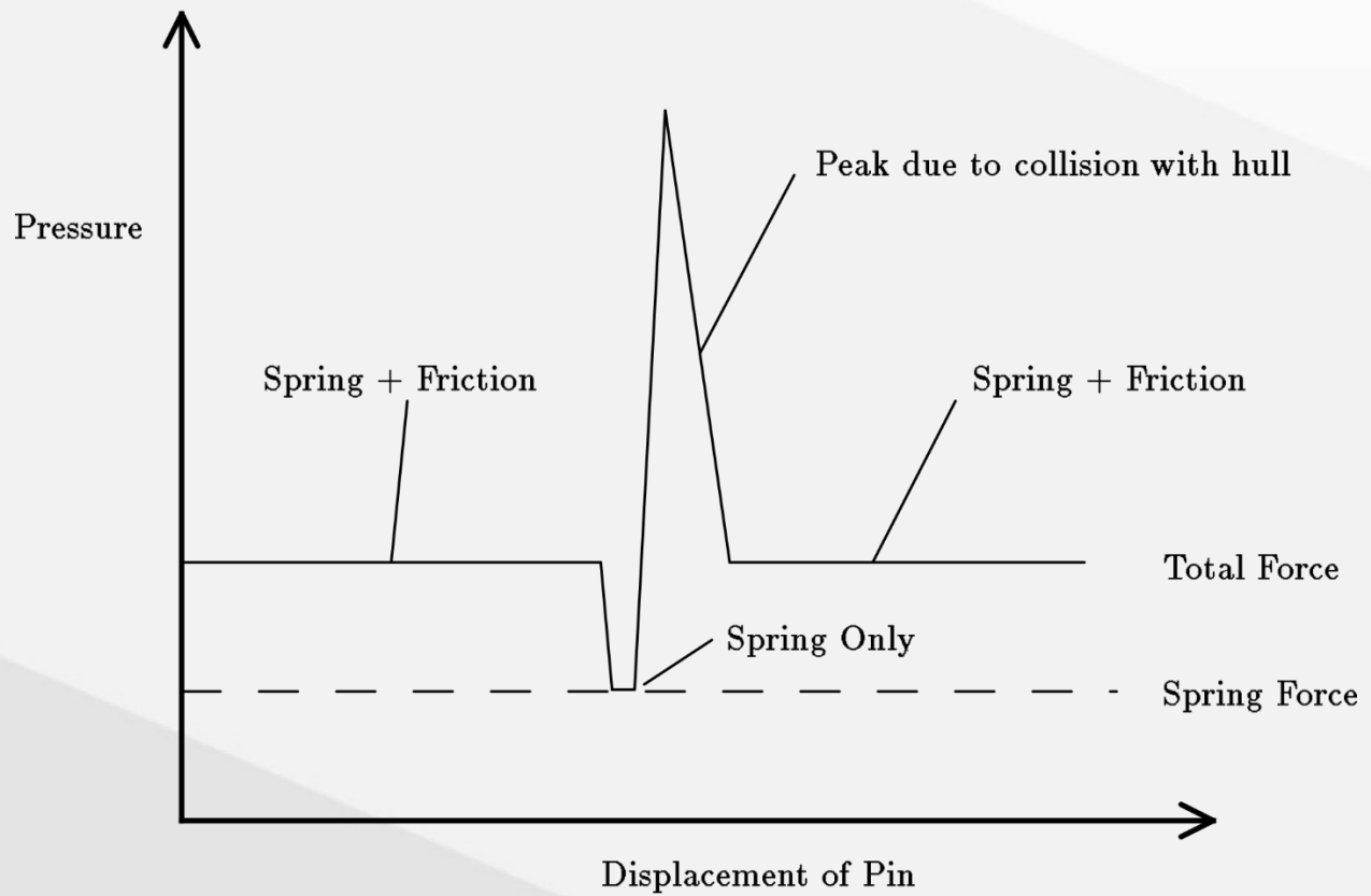
Figure 5.5: Pressure required to move pins
